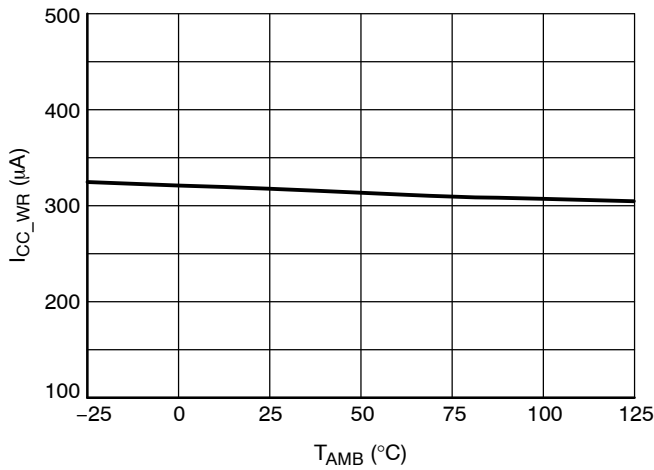
Figure 4. SPD EEPROM Write Current ( I^2\text{C} -bus Idle, TS Shut-down)
